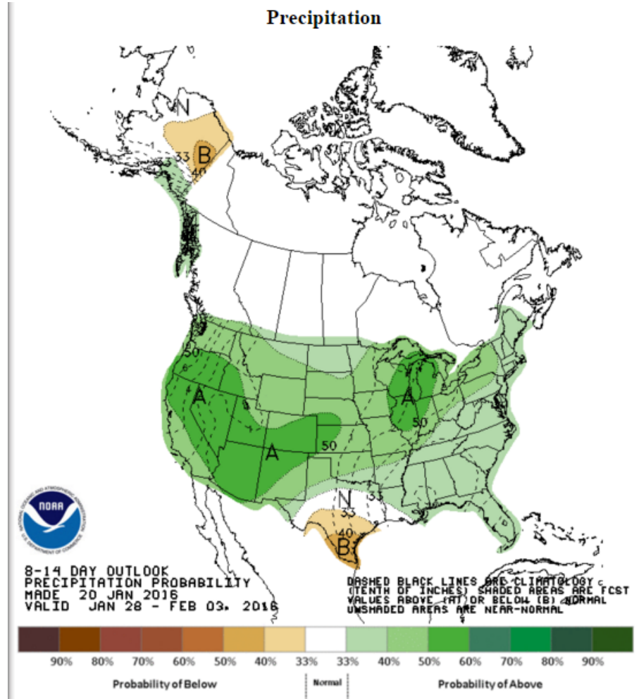
NCEP 8 – 14 day precipitation probability
